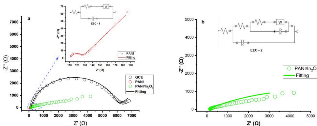
Fig.2 Nyquist plots of the bare GCE, GCE/PANI, and GCE/PANI/In 2 O 3 obtained in 0.1 M PBS buffer containing 5.0 mM Fe(CN) 6 3- /Fe(CN) 6 4- . Insets: a Nyquist plots of the GCE/PANI
